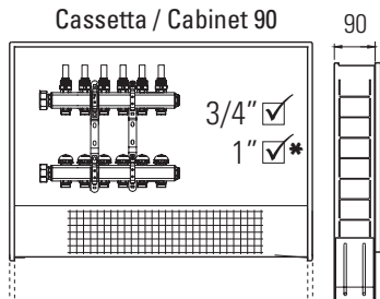
Cassetta / Cabinet 90
