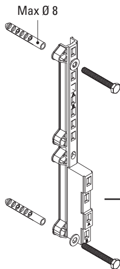
Cassetta / Cabinet 110
